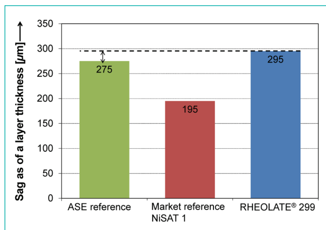
Figure 10: Sag resistance (dft) of the spray-applied waterborne industrial top-coat
