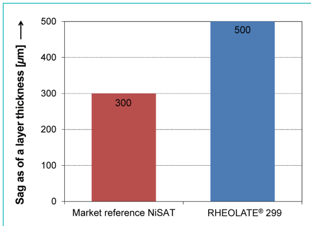
Figure 4: Sag resistance of the waterborne clear-coat formulations
