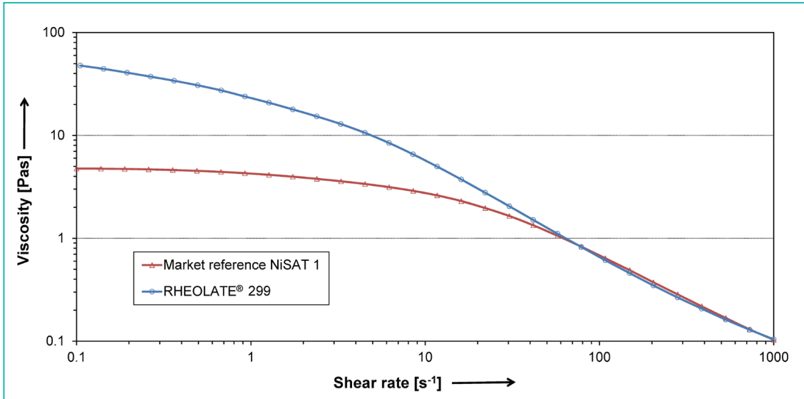
Figure 3: Rheograms of the waterborne clear coat with the RHEOLATE® 299 thickener or the reference PEUPU
