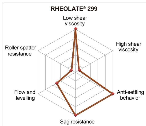
Figure 1: Application properties given by the new generation associative thickener
