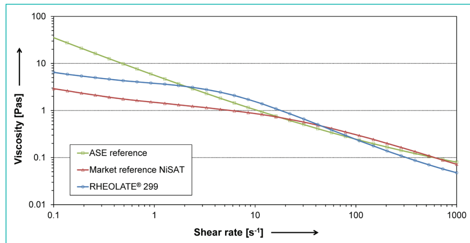
Figure 9: Rheograms of the spray-applied waterborne top-coat thickened with the RHEOLATE® 299, a standard PEUPU, or a bench-mark ASE (30s DIN 4 cup)
