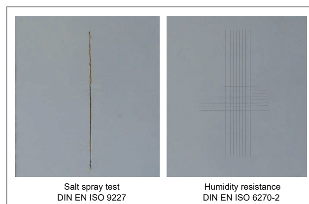
Figure 11: Corrosion and humidity resistance panels. Industrial spray applied top-coat containing the RHEOLATE® 299 associative thickener
