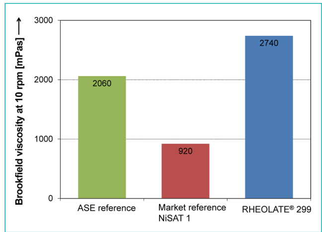
Figure 6: Mid shear viscosity
