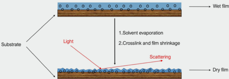
FIGURE 2: Matting effect
