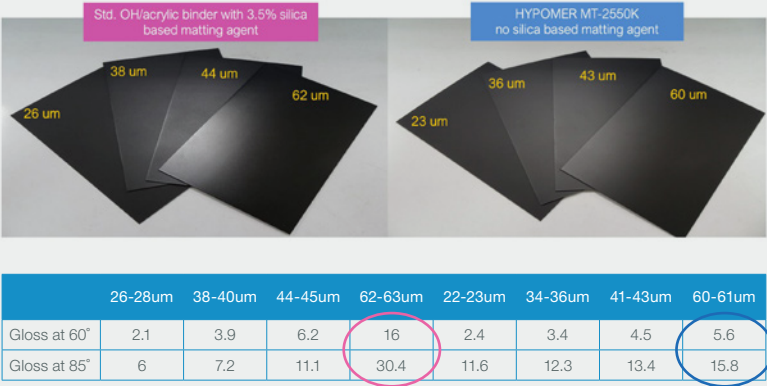
FIGURE 4: Gloss in dependence on the DFT
