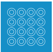
HOMOGENEOUS MATRIX
