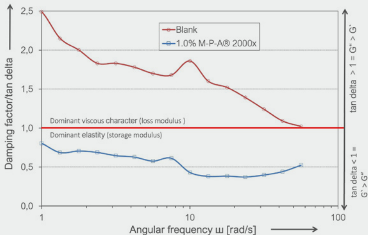
FIGURE 4: Frequency sweep
