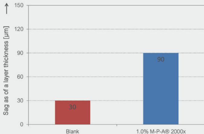
FIGURE 5: Sag control
