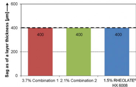
FIGURE 12 RHEOLATE® HX 6008 - acrylic PVC 30% paint
