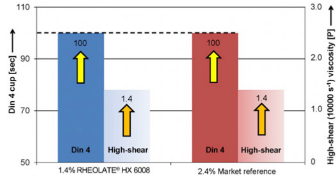
FIGURE 21 Efficiency - acrylic parquet lacquer
