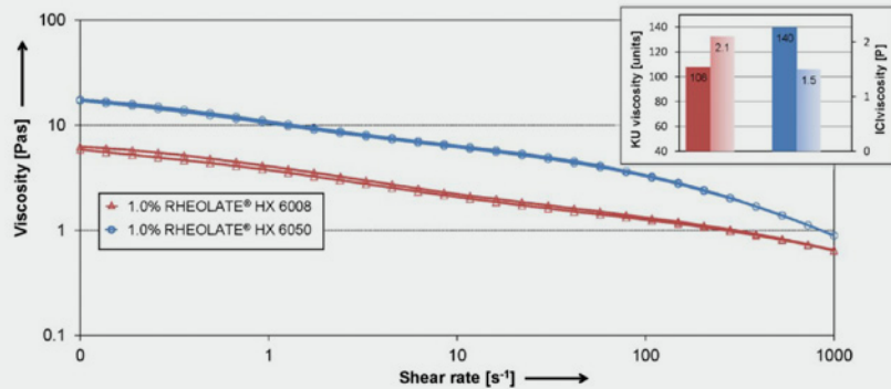
FIGURE 3: Pure acrylic PVC 30% paint
