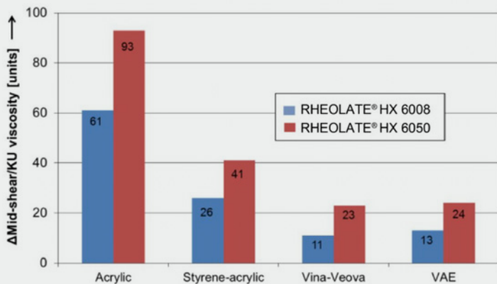
FIGURE 26: High-viscosity increase with 1% of RHEOLATE® HX 6008/6050
