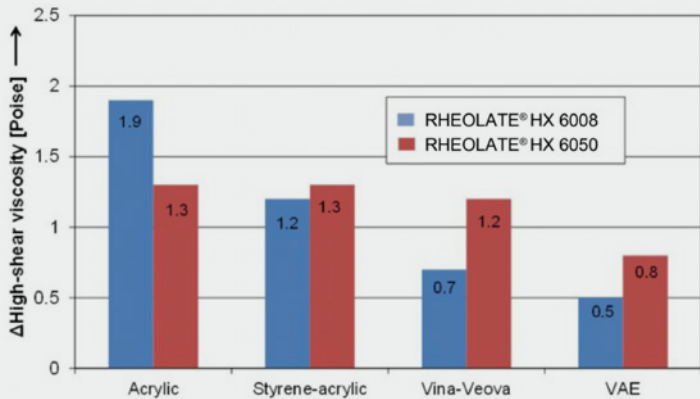
FIGURE 25: High-viscosity increase with 1% of RHEOLATE® HX 6008/6050
