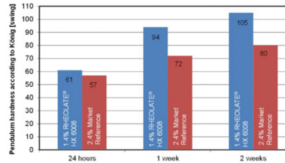
FIGURE 24 Pendulum hardness - acrylic parquet lacquer
