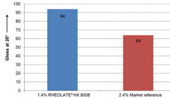
FIGURE 23 Gloss at 20° - acrylic parquet lacquer
