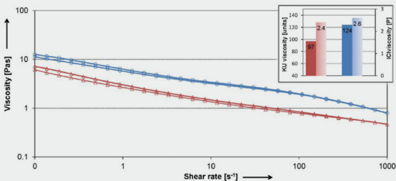
FIGURE 4: Styrene-acrylic PVC 50% paint
