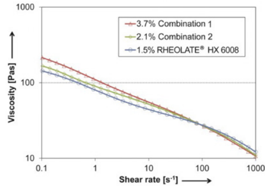
FIGURE 10 RHEOLATE® HX 6008 - acrylic PVC 30% paint
