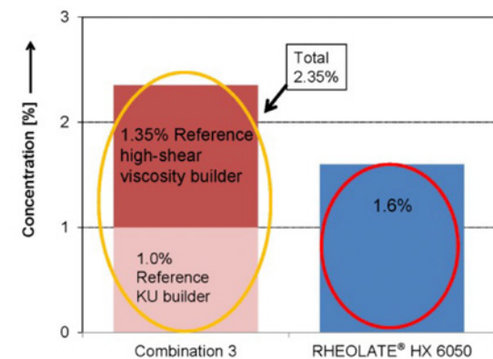
FIGURE 9: RHEOLATE® HX 6050 - VAE based PVC 50%paint
