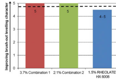
FIGURE 14 RHEOLATE® HX 6008 - acrylic PVC 30% paint
