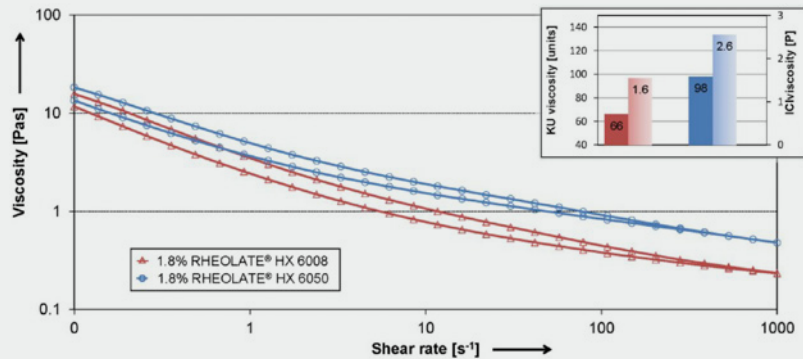
FIGURE 5: Vina-Veova based PVC 50% paint
