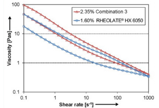
FIGURE 11: RHEOLATE® HX 6050 - VAE based PVC 50% paint
