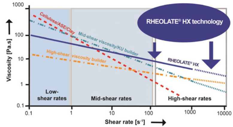
FIGURE 27: Comparison of the provided flow with RHEOLATE® HX 6008/6050
