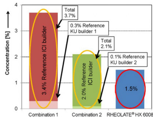
FIGURE 8: RHEOLATE® HX 6008 - acrylic PVC 30% paint
