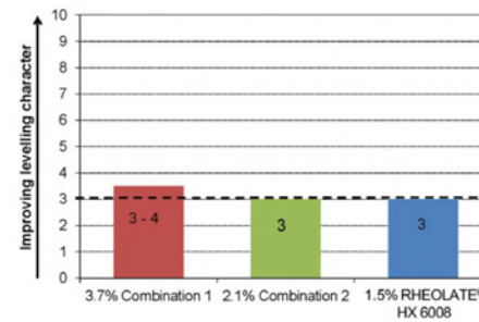
FIGURE 16 RHEOLATE® HX 6008 - acrylic PVC 30% paint
