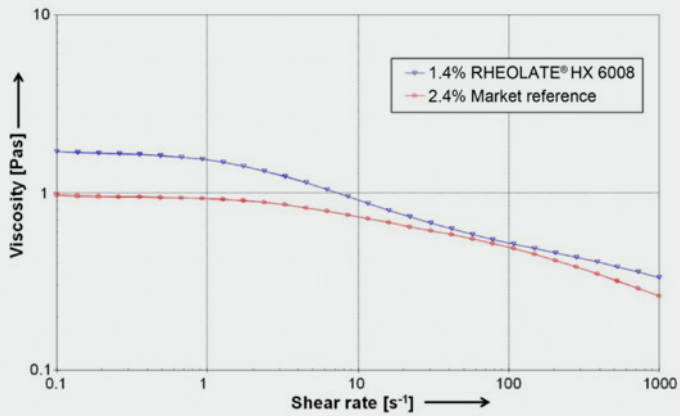
FIGURE 22 Rheograms - acrylic parquet lacquer
