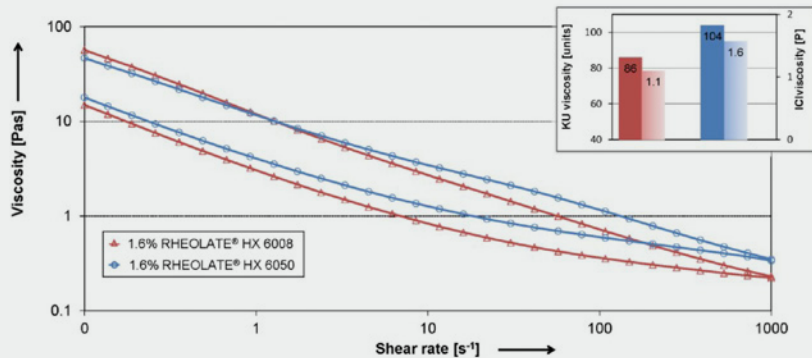
FIGURE 6: Vinyl-acetate-ethylene based PVC 50% paint
