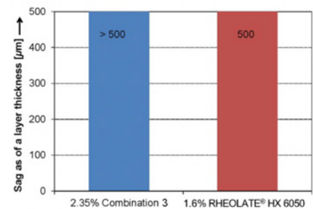
FIGURE 13: RHEOLATE® HX 6050 - VAE based PVC 50% paint
